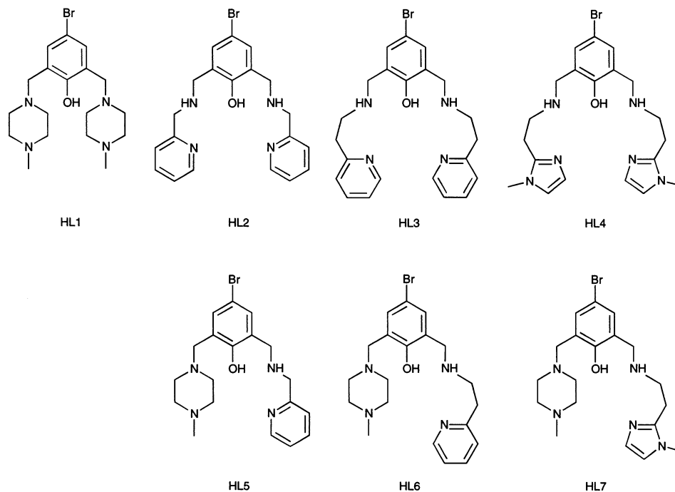
Fig. 11. Schematic structures of the pentadentate symmetric ligands \text{HL}^1 = 4\text{-bromo-2,6-bis(4-methylpiperazin-1-ylmethyl)phenol} , \text{HL}^2 = 4\text{-bromo-2,6-bis((2-pyridylmethyl)aminomethyl)phenol} , \text{HL}^3 = 4\text{-bromo-2,6-bis((2-(2-pyridyl)ethyl)aminomethyl)phenol} and \text{HL}^4 = 4\text{-bromo-2,6-bis((2-(1-methyl-2-imidazolyl)ethyl)aminomethyl)phenol} and asymmetric ligands \text{HL}^5 = 4\text{-bromo-2-(4-methylpiperazin-1-ylmethyl)-6-((2-pyridylmethyl)aminomethyl)phenol} , \text{HL}^6 = 4\text{-bromo-2-(4-methylpiperazin-1-ylmethyl)-6-((2-(2-pyridyl)ethyl)aminomethyl)phenol} and \text{HL}^7 = 4\text{-bromo-2-(4-methylpiperazin-1-ylmethyl)-6-((2-(1-methyl-2-imidazolyl)ethyl)aminomethyl)phenol} [104].
